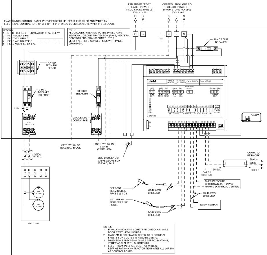
REFRIG - CASE CONTROLLER WIRING DIAGRAM (MEDIUM TEMP TIMED-OFF DEFROST, BOX W/ ONE COIL) SCALE: 1/8" = 1'-0"
