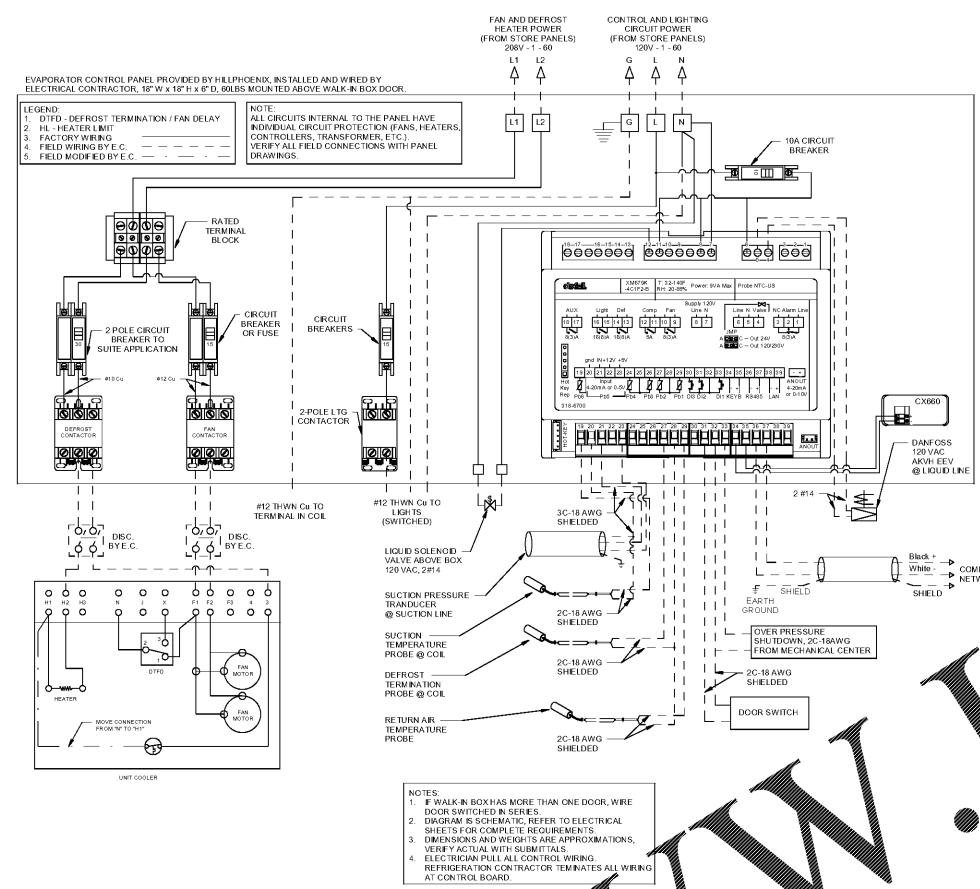
REFRIG - CASE CONTROLLER WIRING DIAGRAM (LOW TEMP ELECTRIC DEFROST, BOX W/ ONE COIL) SCALE: N.T.S.
