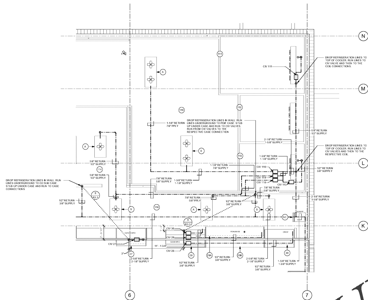
1 ENLARGED MEAT/SEAFOOD/APRONS MT PIPING SCALE: 1/4" = 1'-0"
