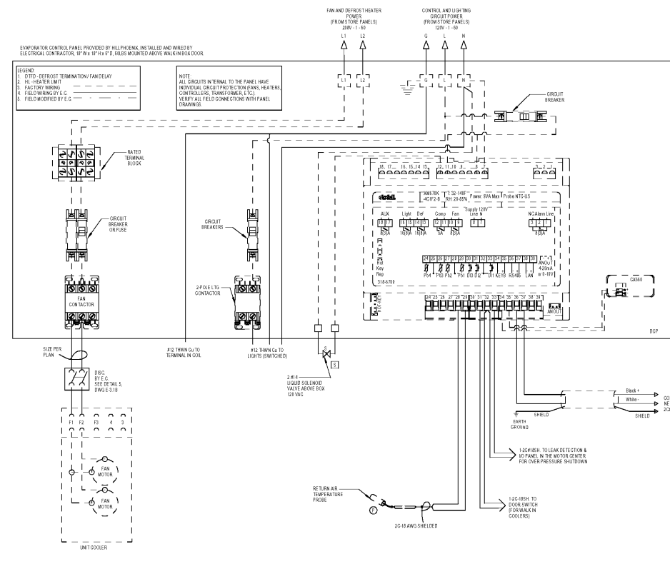
1 DCP WIRING DIAGRAM - MED. TEMP. (TIMED OFF DEFOST, COOLER W/ ONE COIL) SCALE: 1/8" = 1'-0"
