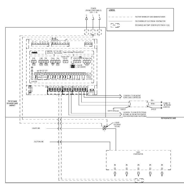
4 CASE WIRING DIAGRAM - MED. TEMP. (TIMED OFF DEFOST, REFRIGERATED CASE) SCALE: 1/8" = 1'-0"
