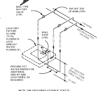
4 PLUMB - PARALLEL HOT WATER LOOP DETAIL SCALE: 1/8\"/>
