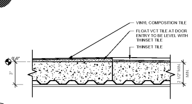
22 MEZZ FLOOR - TILE TO VINYL COMPOSITION TILE SCALE: 3" = 1'-0"
