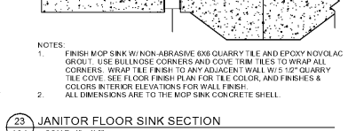
23 JANITOR FLOOR SINK SECTION SCALE: 1" = 1'-0"
