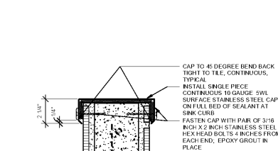
24 JANITOR FLOOR SINK CURB DETAIL SCALE: 3" = 1'-0"
