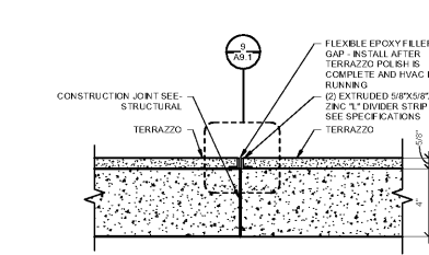
8 TERRAZZO CONSTRUCTION JOINT SCALE: 3" = 1'-0"
