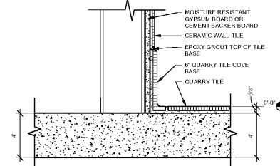
7 QUARRY TILE TO STUD WALL SCALE: 3" = 1'-0"
