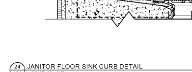
24 JANITOR FLOOR SINK CURB DETAIL SCALE: 3" = 1'-0"
