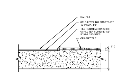
3 QUARRY TILE TO CARPET SCALE: 3" = 1'-0"
