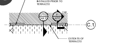
27 ENLARGED FINISH PLAN - AUTO DOORS SCALE: 1/2" = 1'-0"
