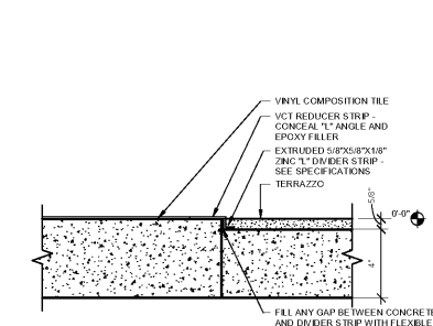
20 TERRAZZO TO VINYL COMPOSITION TILE SCALE: 3" = 1'-0"
