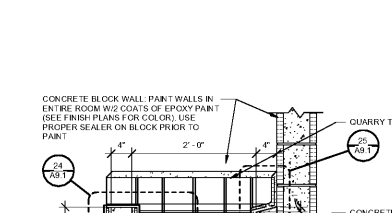
23 JANITOR FLOOR SINK SECTION SCALE: 1" = 1'-0"
