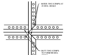
12 TERRAZZO METAL STRIPS AT EXPANSION JOINT SCALE: 6" = 1'-0"
