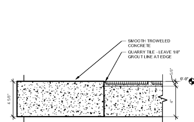
5 QUARRY TILE TO CONCRETE FLOOR SCALE: 3" = 1'-0"
