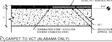
26 CARPET TO VCT (ALABAMA ONLY) SCALE: 3" = 1'-0"
