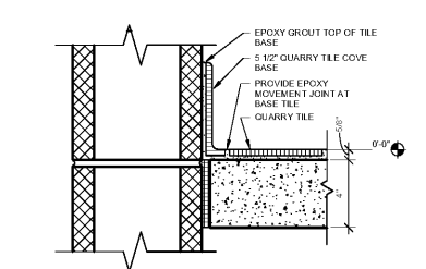
4 QUARRY TILE TO CMU WALL SCALE: 3" = 1'-0"
