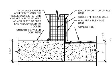
6 QUARRY TILE TO COOLER WALL SCALE: 3" = 1'-0"
