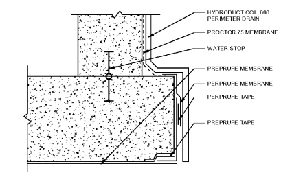
ELEVATOR PIT WATERPROOFING DETAIL SCALE: 1" = 1'-0"
