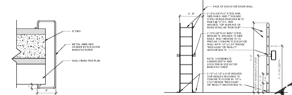
ELEVATOR DOOR JAMB / HEAD SCALE: 3" = 1'-0"
