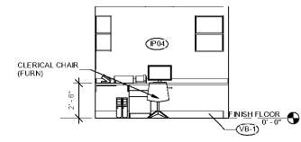
3 DEPARTMENT OFFICE SCALE: 1/4" = 1'-0"
