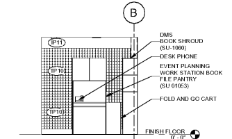
6 EVENT PLANNING SCALE: 1/4" = 1'-0"
