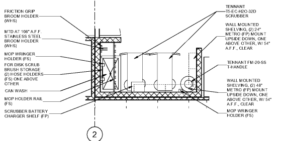
13 ARCH - ENLARGED MOP ROOM SCALE: 1/4" = 1'-0"
