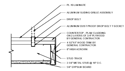
6 PHARMACY ROLLING GRILLE COUNTER LOCK SCALE: 3" = 1'-0"
