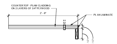
7 PHARMACY COUNTERTOP SCALE: 1 1/2" = 1'-0"
