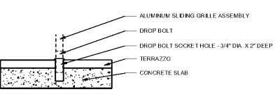
8 PHARMACY ROLLING GRILLE FLOOR LOCK SCALE: 3" = 1'-0"
