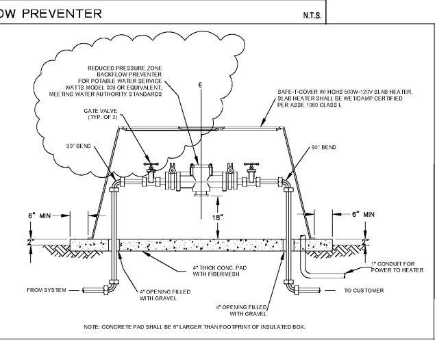
2" & 2.5" REDUCED PRESSURE ZONE BACKFLOW PREVENTER N.T.S.
