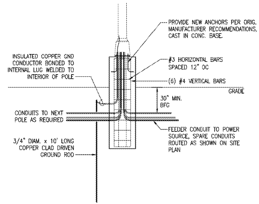
POLE BASE AND FIXTURE RE-MOUNTING DETAIL SCALE: N.T.S.
