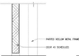
12 SILL AT INTERIOR DOOR SCALE: 3"=1'-0"
