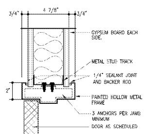
14 HEAD AT INTERIOR DOOR SCALE: 3"=1'-0"
