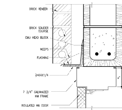
7 HEAD AT EXTERIOR DOOR SCALE: 3"=1'-0"
