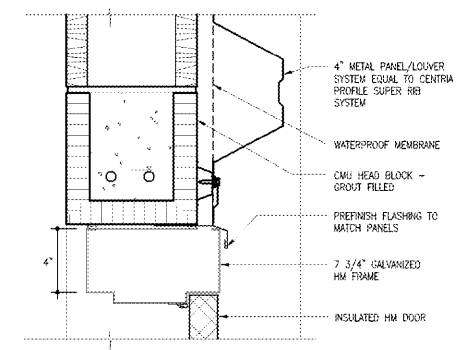
15 DOOR HEAD DETAIL SCALE: 3"=1'-0"
