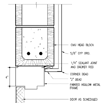
10 HEAD AT INTERIOR DOOR SCALE: 3"=1'-0"
