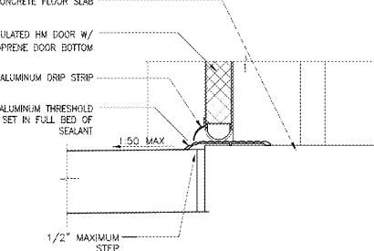
4 SILL AT EXTERIOR DOOR SCALE: 3"=1'-0"
