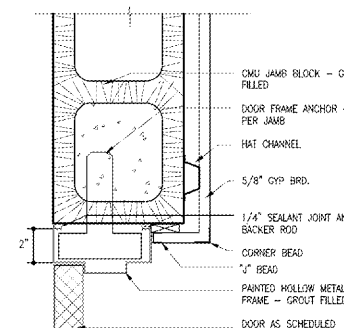
9 JAMB AT INTERIOR DOOR SCALE: 3"=1'-0"
