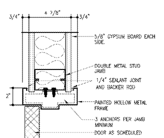
13 JAMB AT INTERIOR DOOR SCALE: 3"=1'-0"
