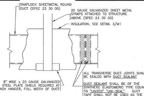
ROUND DUCT INSULATION HANGER SHIELD N.T.S.
