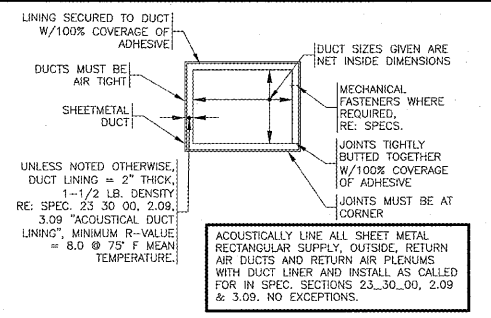
RECTANGULAR DUCT LINER INSULATION N.T.S.
