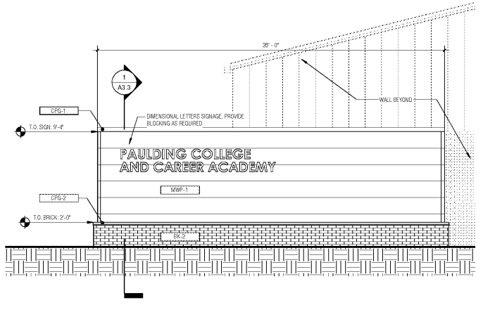
7 ENLARGED ELEVATION - SIGN A2.2 SCALE: 1/4" = 1'-0"
