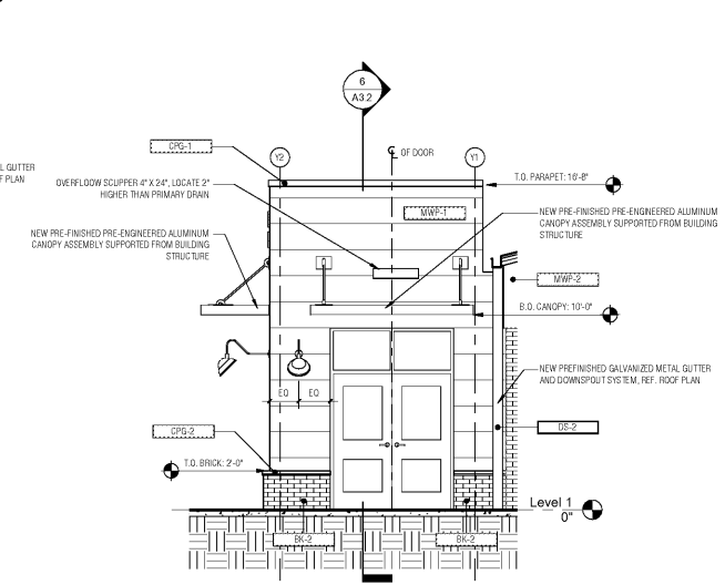
6 ENLARGED ELEVATION - ENTRANCE VESTIBULE - WEST A2.2 SCALE: 1/4" = 1'-0"
