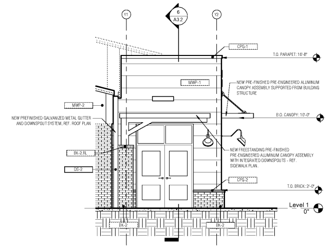
2 ENLARGED ELEVATION - ENTRANCE VESTIBULE - EAST A2.2 SCALE: 1/4" = 1'-0"
