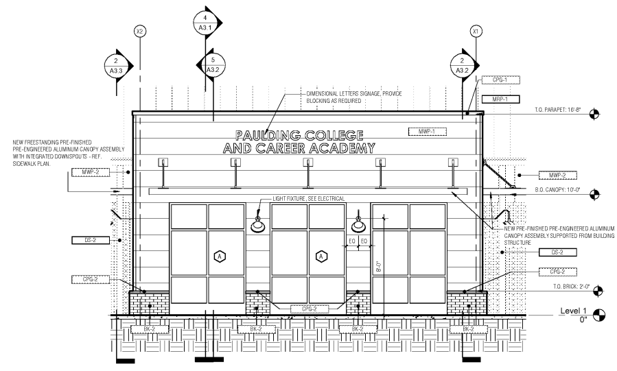
1 ENLARGED ELEVATION - ENTRANCE VESTIBULE - NORTH A2.2 SCALE: 1/4" = 1'-0"
