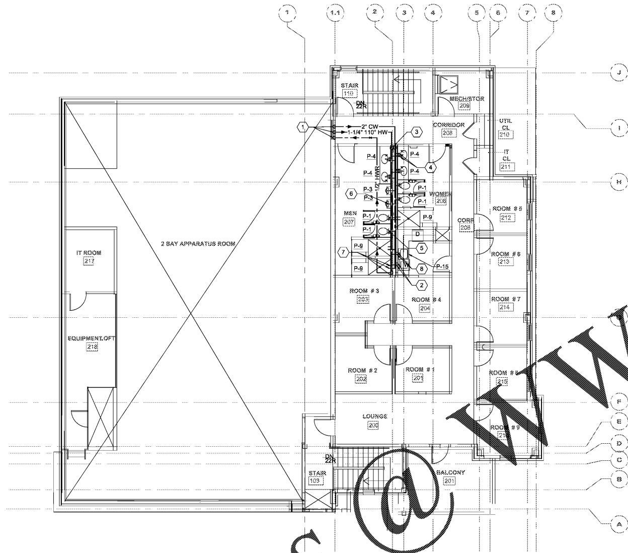
1 PLUMBING - DOMESTIC WATER - SECOND FLOOR PLAN P101 SCALE: 1/8" = 1'-0"
