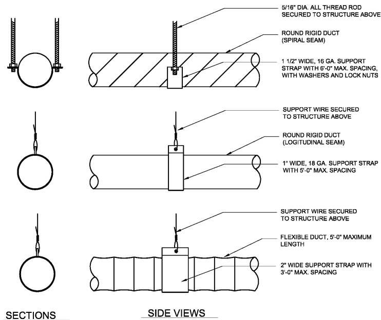
1 ROUND DUCT SUPPORT
