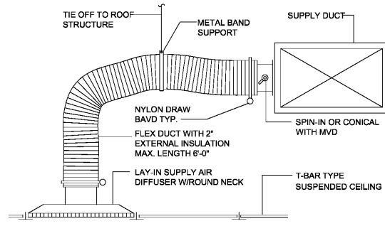
5 SUPPLY AIR DIFFUSER
