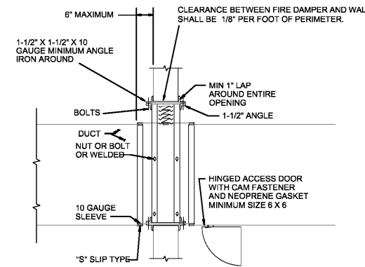
5 FIRE DAMPER M-500 NO SCALE
