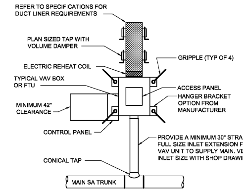
8 FAN POWERED TERMINAL UNIT DETAIL M-500 SCALE: NONE
