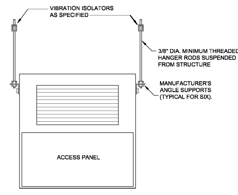
7 FAN POWERED TERMINAL MOUNTING DETAIL M-500 SCALE: NONE
