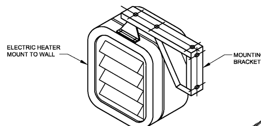
3 ELECTRIC UNIT HEATER DETAIL M-500 SCALE: NONE
