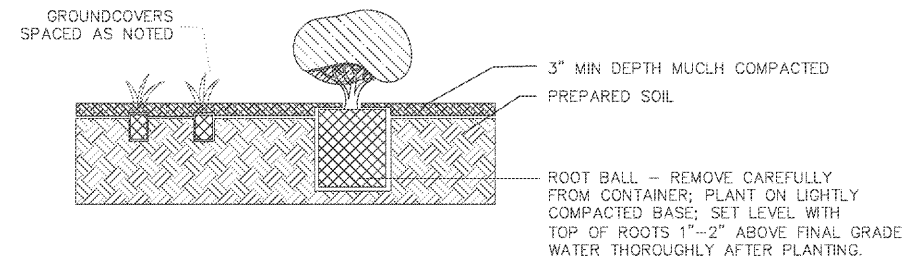
1 SHRUB & GROUNDCOVER PLANTING DETAIL SCALE: NONE
