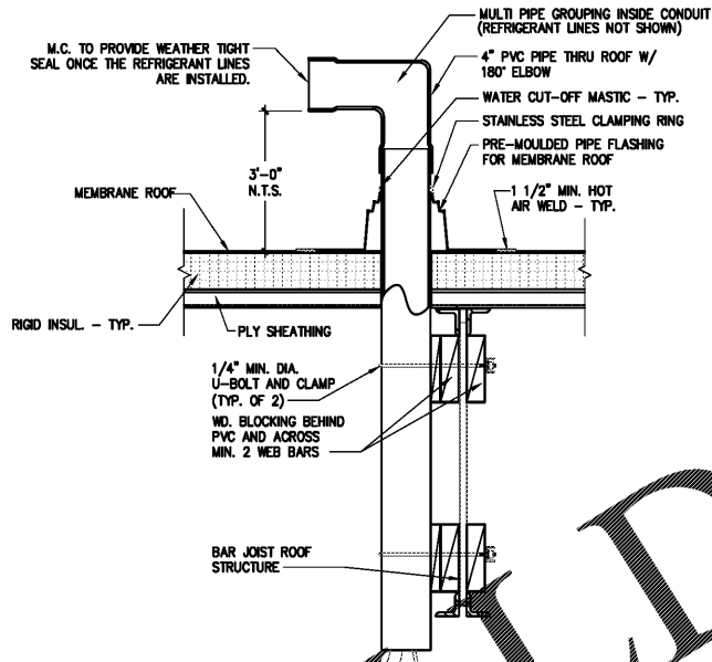
1 REFRIGERANT CONDUIT PENETRATION DETAIL SCALE: 1 1/2" = 1'-0"
