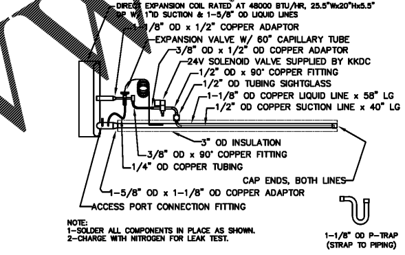
3 COOLING TUNNEL REFRIGERANT PIPING DETAIL SCALE: 1 1/2" = 1'-0" (PER KK EQUIPMENT DEPT.)
