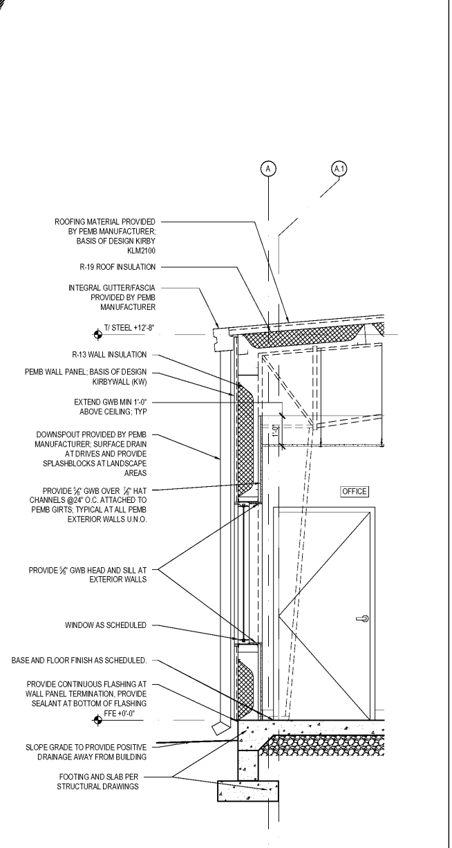
D 1/2" 1'-0" WALL SECTION
