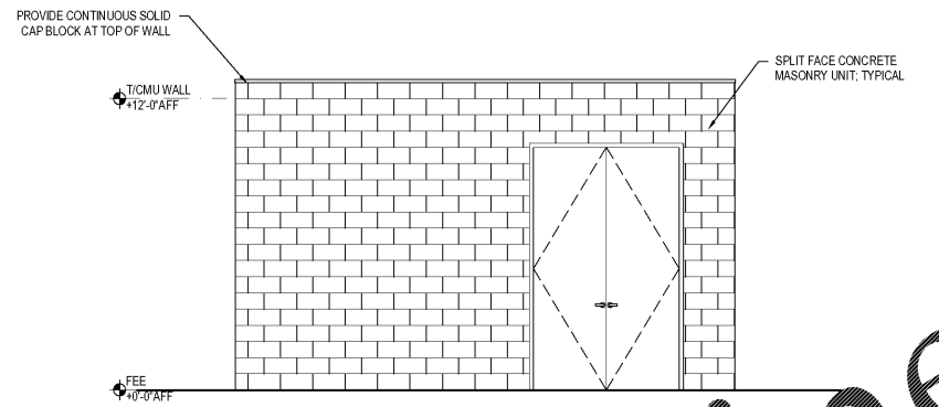
B 1/4" 1'-0" BUNKER ELEVATION
