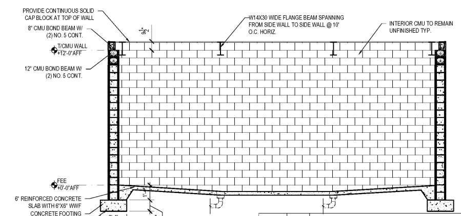
F 1/4" 1'-0" BUNKER SECTION
