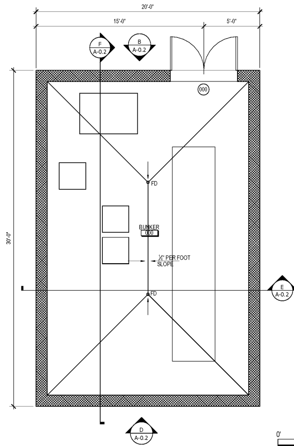
A 1/4" 1'-0" BUNKER PLAN
