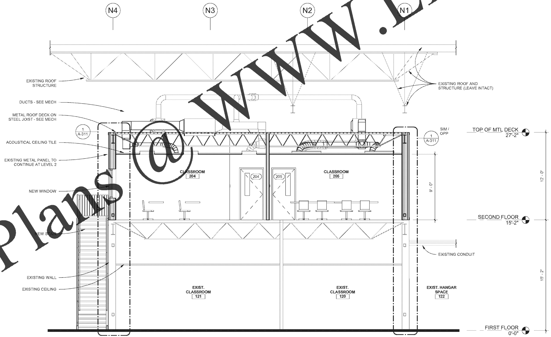
1 A-301 BUILDING SECTION 1/4" = 1'-0" 0 5 10 FT
