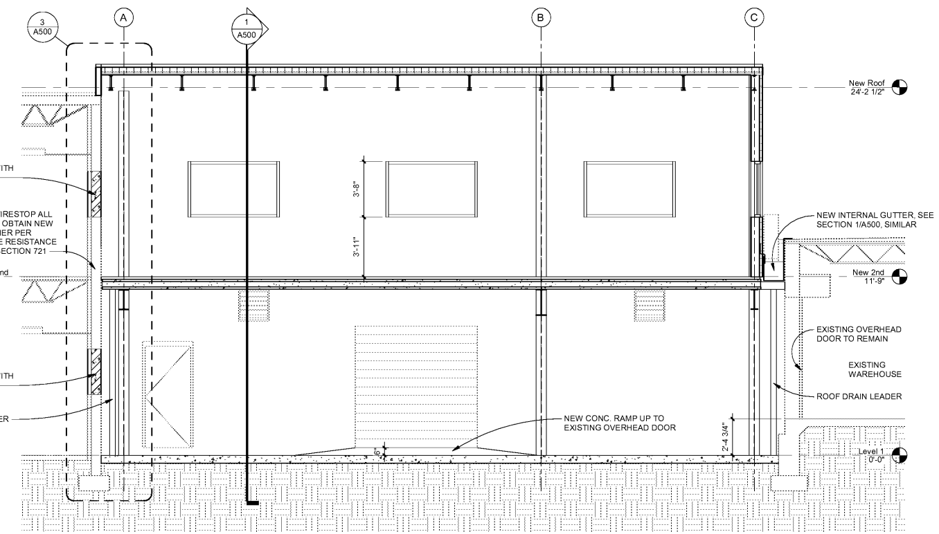
3 BUILDING SECTION SCALE: 1/4" = 1'-0"
