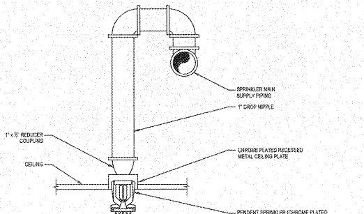
TYPICAL DROP TO PENDENT SPRINKLER SCALE: NONE
