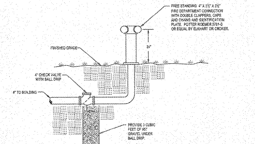
FIRE DEPARTMENT CONNECTION DETAIL SCALE: NONE
