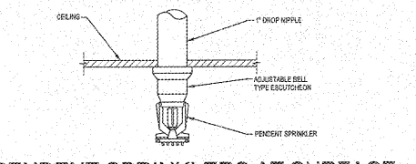
PENDENT SPRINKLERS AT SURFACE MOUNTED LIGHT FIXTURES SCALE: NONE
