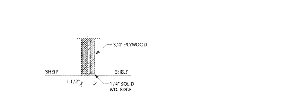
13 WALL SHELF UNIT DETAIL SCALE: 3\"/>
