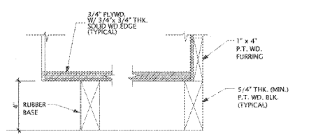
10 BASE SHELVING UNIT SCALE: 3\"/>
