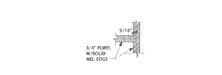
19 SHELF DETAIL SCALE: 3\"/>
