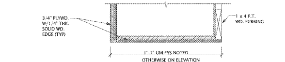
2 COUNTERTOP/ BASE CABINET SECTION SCALE: 3\"/>
