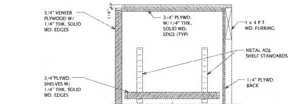
1 WALL CABINET SECTION SCALE: 3\"/>
