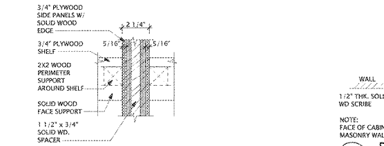
22 INSTR STOR SHELF DETAIL SCALE: 3\"/>
