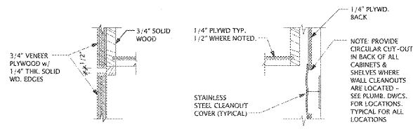
4 BASE CABINET SECTION SCALE: 3\"/>
