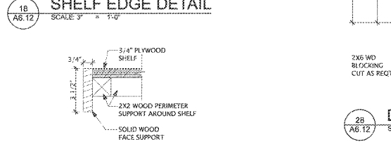
20 INSTR STOR SHELF DETAIL SCALE: 3\"/>
