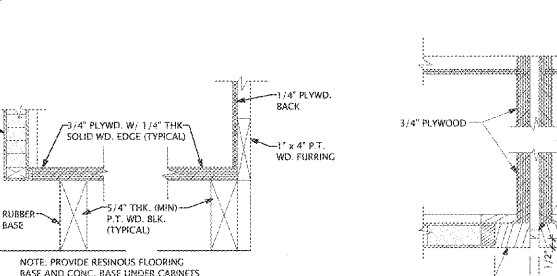
26 STORAGE CAB DETAIL SCALE: 3\"/>
