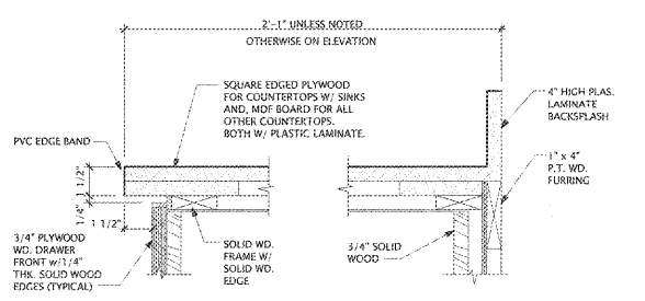
3 BASE CABINET DRAWER SCALE: 3\"/>
