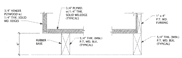
5 BASE WALL CAB DETAIL SCALE: 3\"/>
