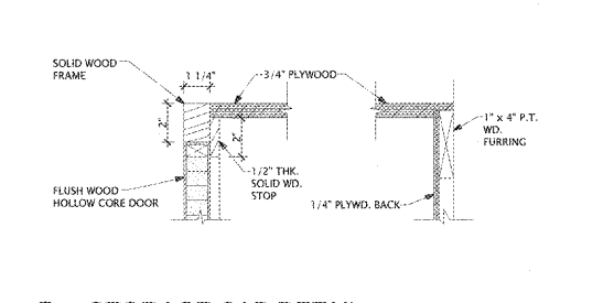
23 STORAGE CAB DETAIL SCALE: 3\"/>
