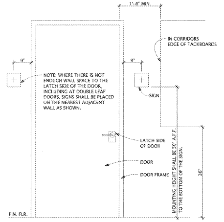
7 MOUNTING LOCATION AND HEIGHT NOT TO SCALE
