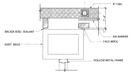
2 PLAN DETAIL SCALE: 3/4" = 1'-0"
