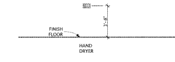
5 TYP. TOILET ACCESSORY MTG HGTS SCALE: 1/4" = 1'-0"
