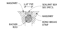
2 PLAN DETAIL SCALE: 3/4" = 1'-0"
