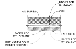
4 PLAN DETAIL SCALE: 3/4" = 1'-0"
