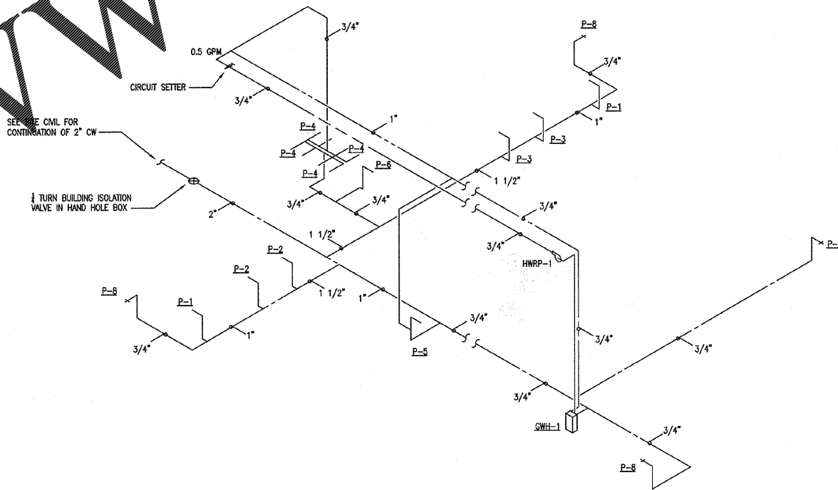
2 HOT AND COLD WATER RISER P201 NO SCALE
