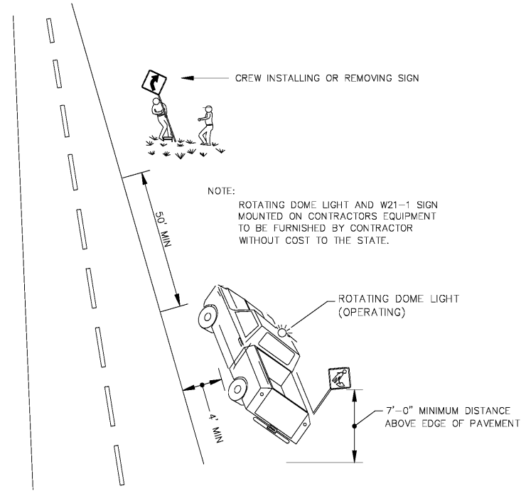
TYPICAL METHOD FOR INSTALLING OR REMOVING CONSTRUCTION SIGNS
