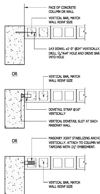
5 MASONRY WALL DETAIL TO CONCRETE COLUMN OR WALL
