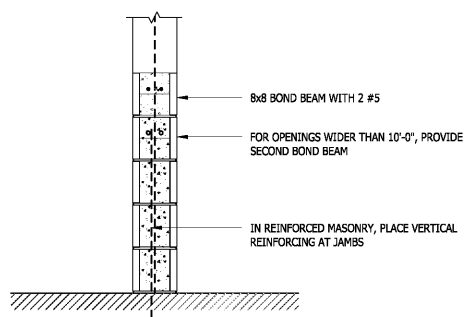
10 TYPICAL MASONRY SILL DETAIL
