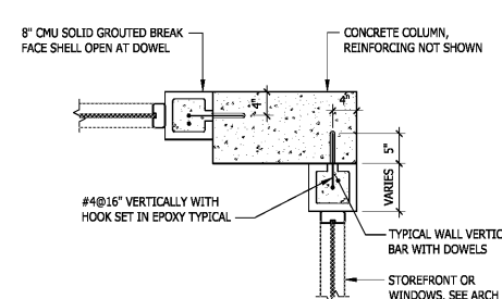
11 MASONRY JAMB TO CONCRETE COLUMN PLAN DETAIL
