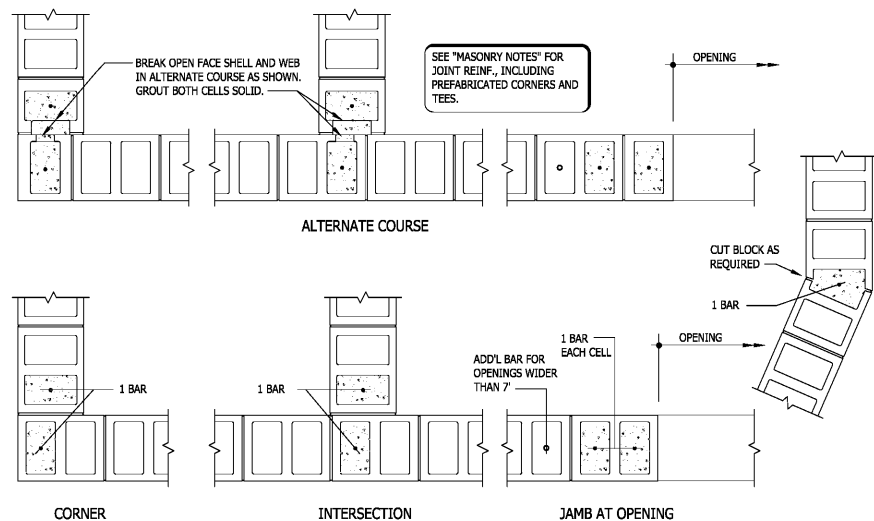
1 12" MASONRY WALL REINFORCING WITH SINGLE REINFORCEMENT
