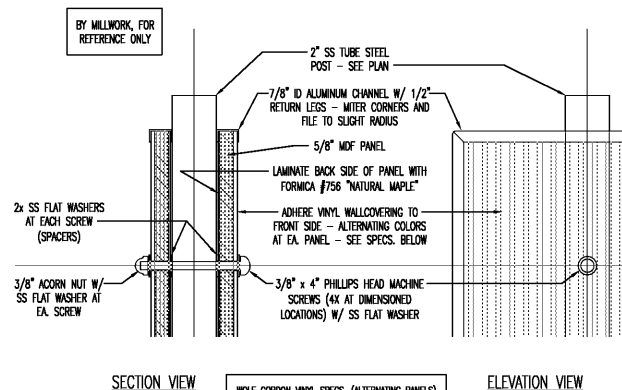
04 DINING ROOM DIVIDER LOW WALL SCALE: 3"=1'-0"
