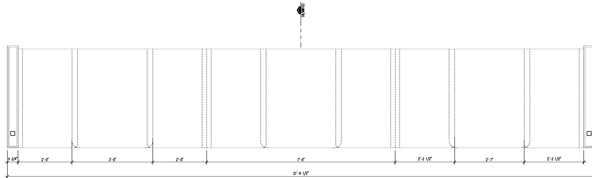
01 PLAN VIEW OF BOOTHS SCALE: 1"=1'-0"
