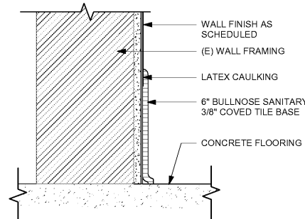
3 TILE BASE AT EXTERIOR WALL Scale: 3" = 1'-0"
