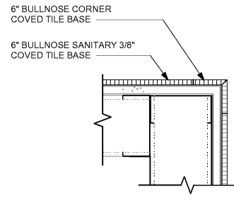
6 TILE BASE AT OUTSIDE CORNER Scale: 3" = 1'-0"
