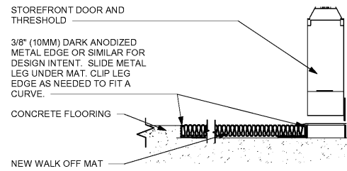
1 TRANSITION - CONCRETE TO WALK OFF MAT Scale: 3" = 1'-0"
