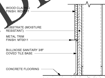
8 CLADDING AT TILE BASE Scale: 3" = 1'-0"
