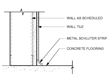
5 METAL SCHLUTER AT RESTROOM WALL Scale: 3" = 1'-0"
