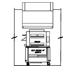
9 BROILER ELEVATION
