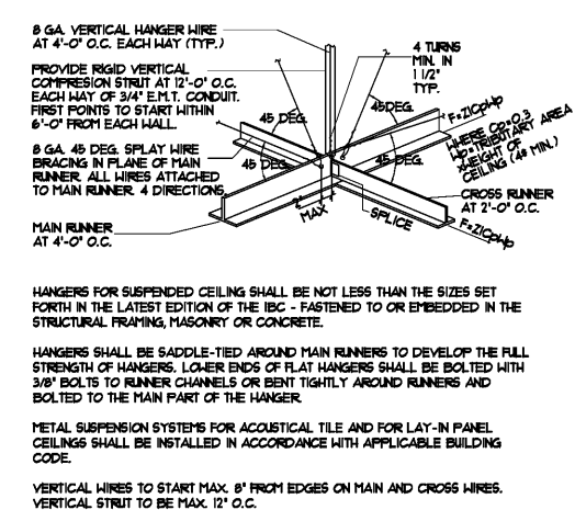
(E) CEILING BRACING DETAIL SCALE: NOT TO SCALE
