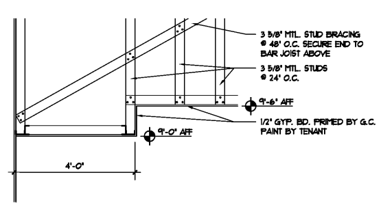
(C) CEILING SECTION SCALE: 1/2" = 1'-0"
