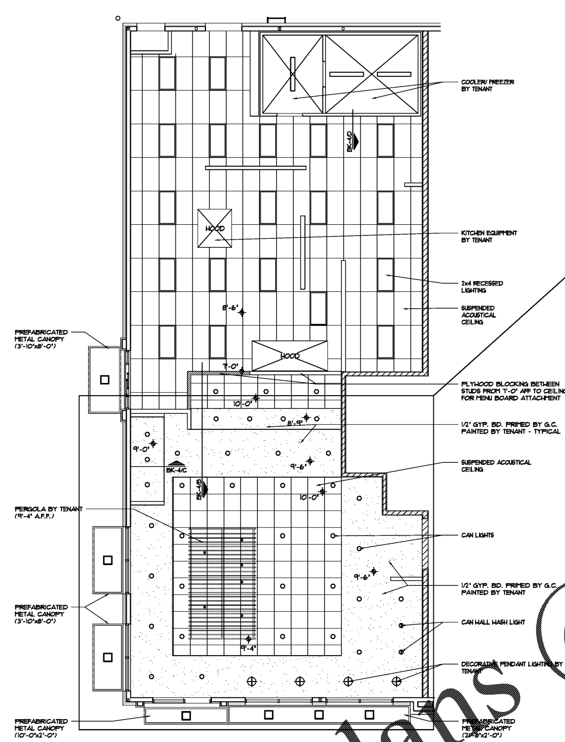
(A) REFLECTED CEILING PLAN SCALE: 3/16" = 1'-0"
