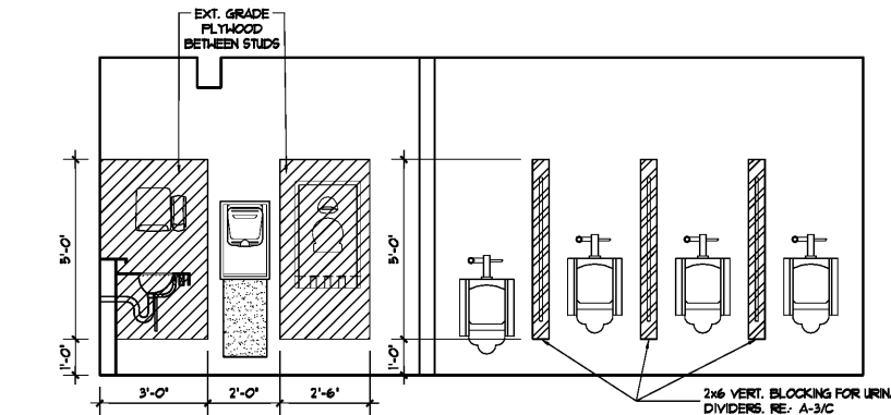
A MEN'S RESTROOM SCALE 3/8" = 1'-0"
