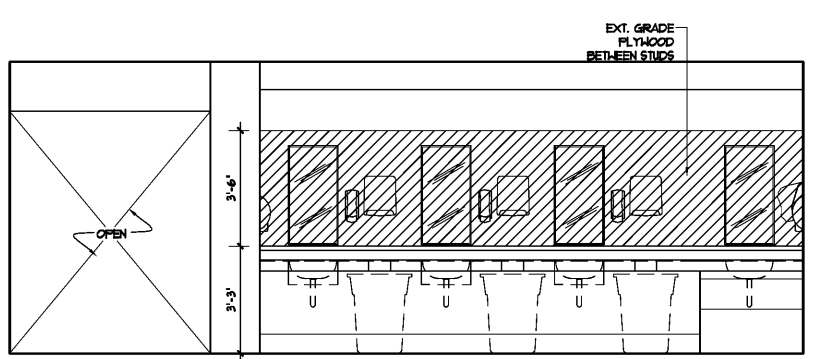
E MEN'S RESTROOM SCALE 3/8" = 1'-0"
