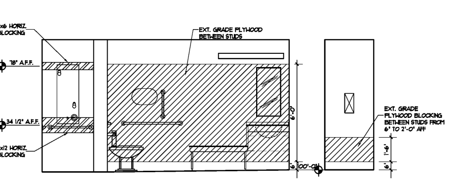
M SHOWER SCALE 3/8" = 1'-0"
