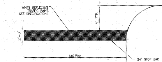
STOP BAR AND PAVEMENT MARKINGS DETAIL N.T.S. CS06
