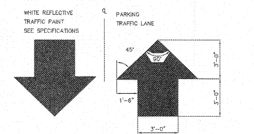
DIRECTIONAL ARROW DETAIL N.T.S. CS08
