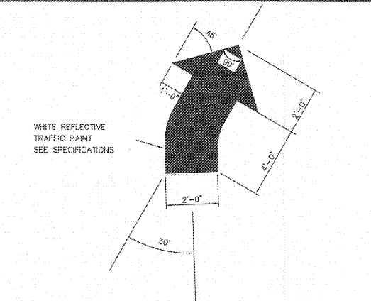
DIRECTIONAL "TURN" ARROW DETAIL N.T.S. CS09
