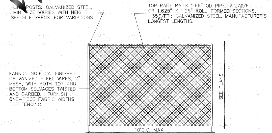
CHAIN LINK FENCE DETAIL NO SCALE CS06
