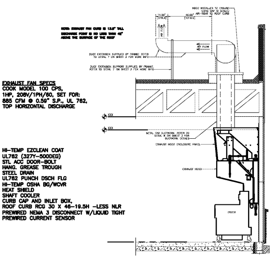
5 FRYER HOOD EXHAUST FAN DETAIL SCALE: NO SCALE
