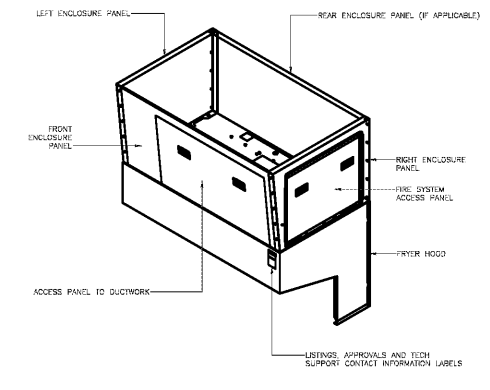
2 HOOD ENCLOSURE DETAIL SCALE: NO SCALE
