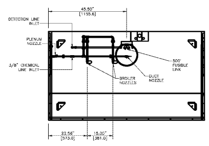
1 FIRE SUPPRESSION PIPING DETAIL SCALE: NO SCALE
