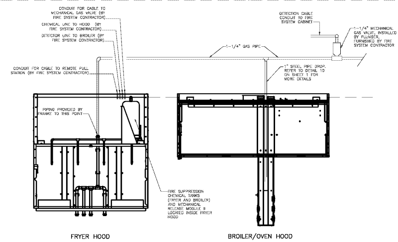
1 FIRE SUPPRESSION PIPING DETAIL SCALE: NO SCALE
