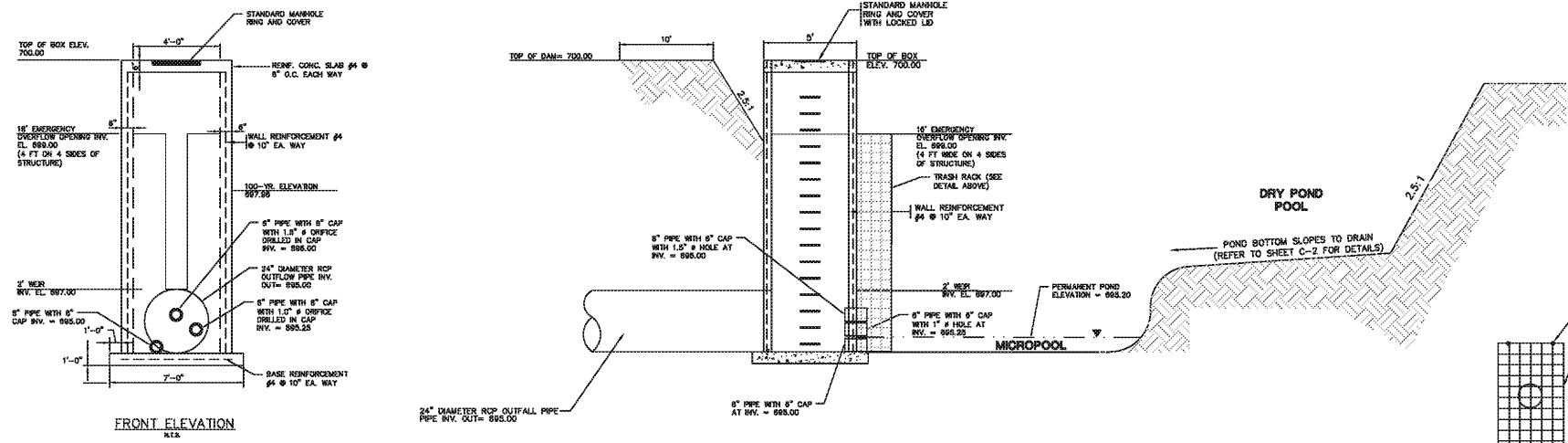
OUTLET CONTROL STRUCTURE DRY DETENTION BASIN (ST2) N.T.S.
