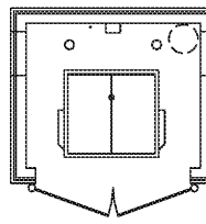
DUMPSTER PLAN SCALE: 1/4" = 1'-0"
