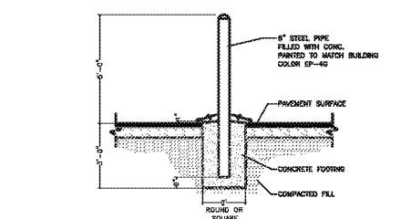
TYPICAL GUARD POST SCALE: NO SCALE JULY 8, 2010
