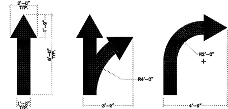
PAINTED TRAFFIC ARROWS SCALE: N.T.S. JULY 15, 1999
