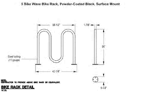
BIKE RACK DETAIL N.T.S.
