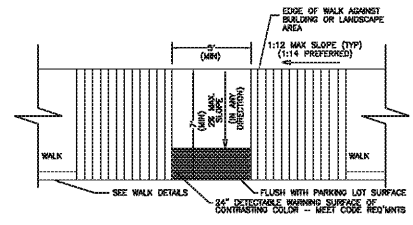
ACCESSIBLE PARKING RAMP SCALE: NO SCALE OCTOBER 28, 2010
