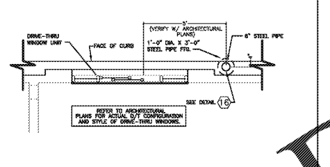
GUARD POST @ D/T WINDOW SCALE: NO SCALE OCTOBER 28, 2010
