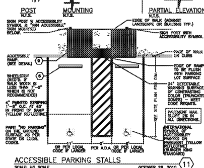
ACCESSIBLE PARKING STALLS SCALE: NO SCALE OCTOBER 28, 2010
