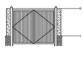
DUMPSTER FRONT ELEVATION SCALE: 1/4" = 1'-0"
