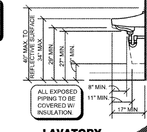
11 LAVATORY CLEARANCES A4.1 SCALE: 1/2" = 1'-0"
