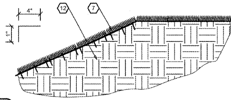
1 SOD DETAIL L1.2 SCALE: 3/4" = 1'-0"
