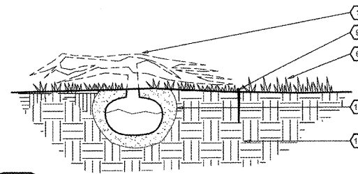
4 SMALL SHRUB DETAIL L1.2 SCALE: 3/4" = 1'-0"
