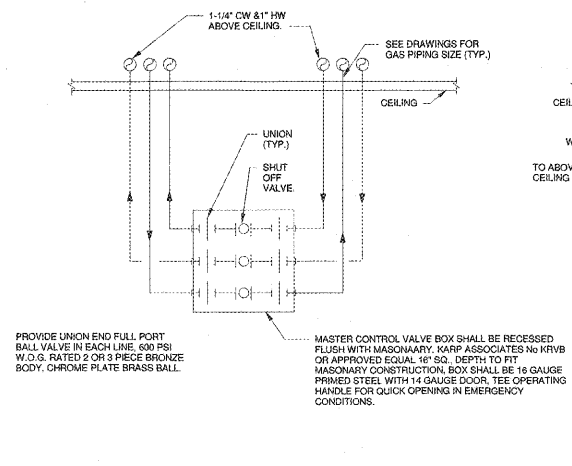
3 P6.1 MASTER SHUT OFF BOX 1/8\"/>
