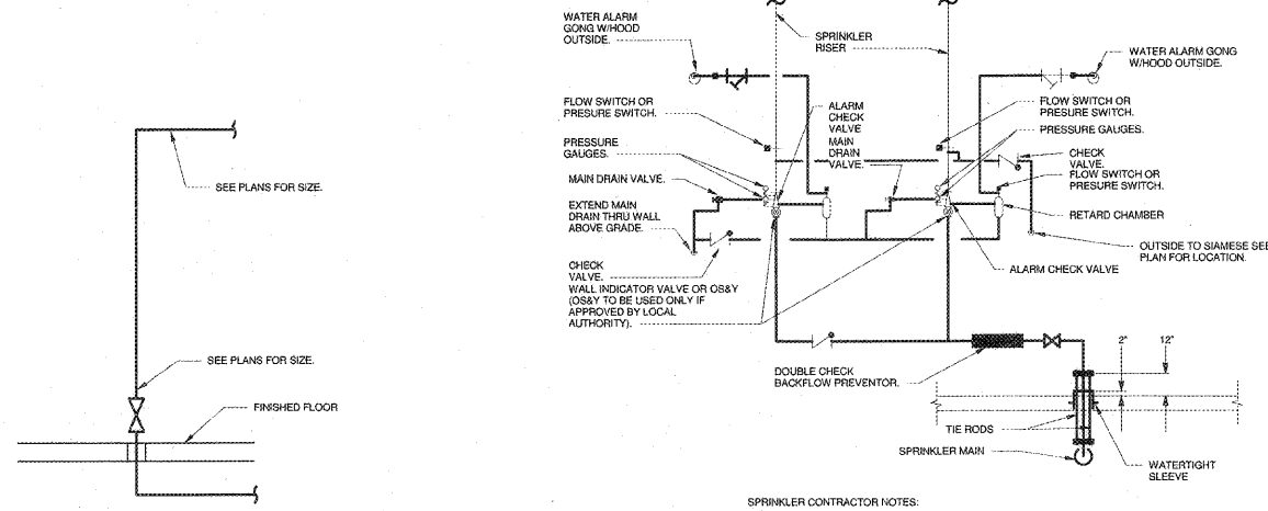
1 P6.1 WATER RISER DIAGRAM NONE
