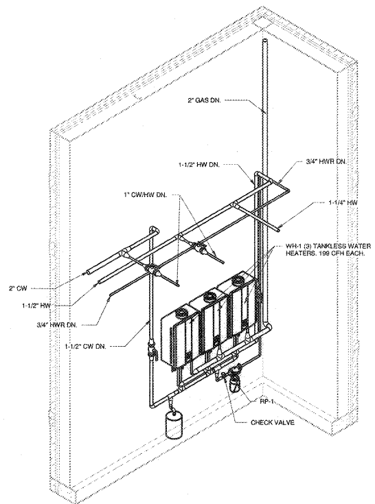
2 WATER HEATER RISER LOWER LEVEL
