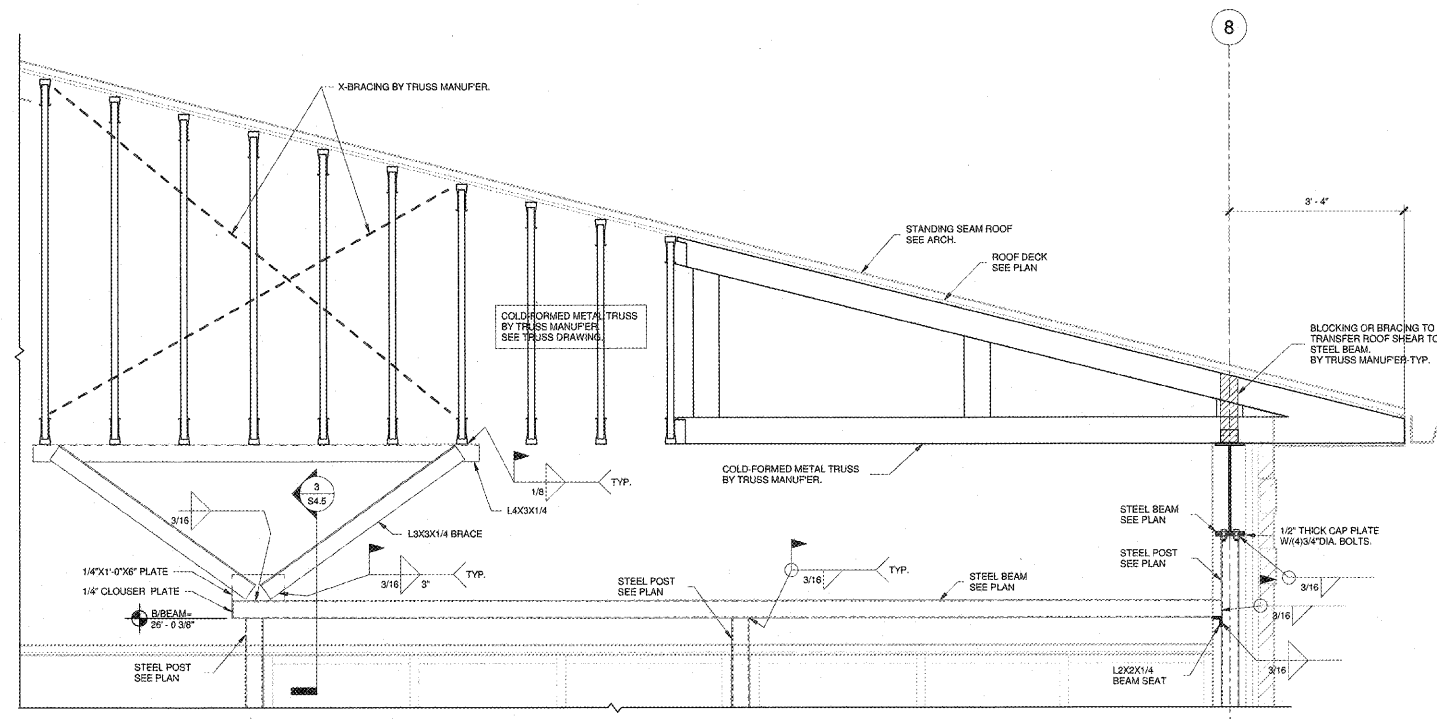
Section 90 3/4" = 1'-0"
