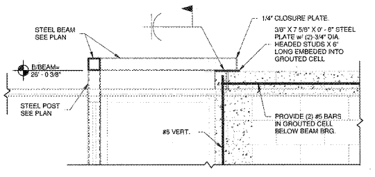
Section 69 3/4" = 1'-0"
