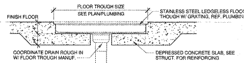
FLOOR TROUGH DETAIL 1" = 1'-0"
