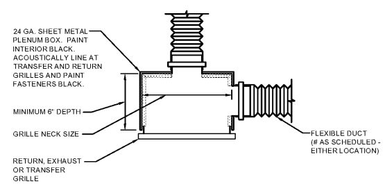
GRILLE PLENUM BOX DETAIL NO SCALE
