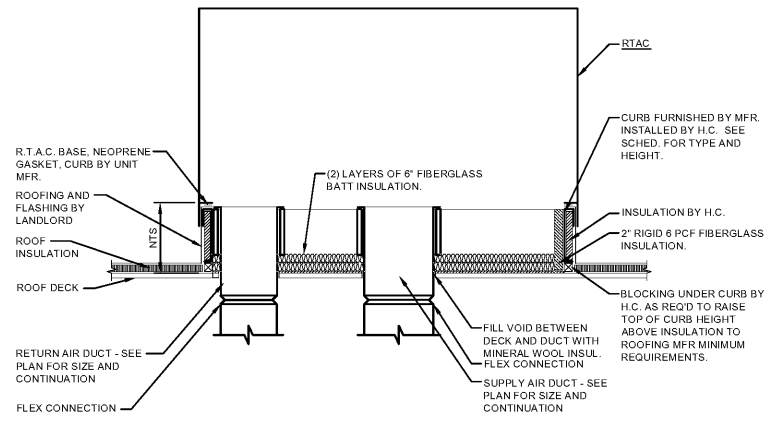
TYPICAL RTAC AND CURB DETAIL NO SCALE
