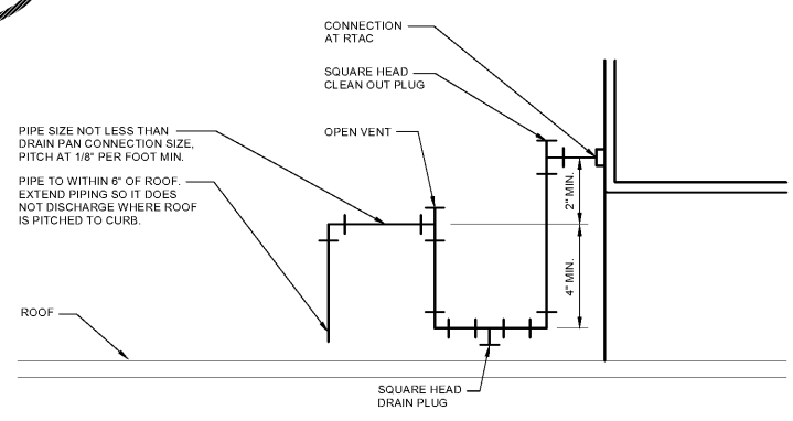
RTAC CONDENSATE DRAIN TRAP PIPING DETAIL NO SCALE
