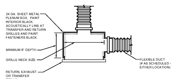
GRILLE PLENUM BOX DETAIL NO SCALE
