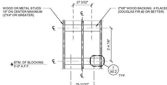
6 BLOCKING DETAIL A5.2 NOT TO SCALE
