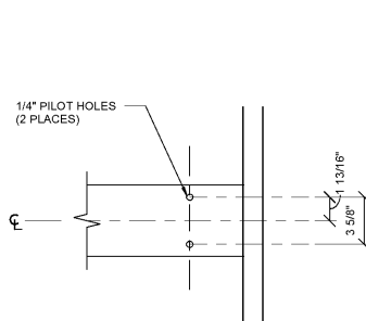
7 BLOCKING DETAIL A5.2 NOT TO SCALE
