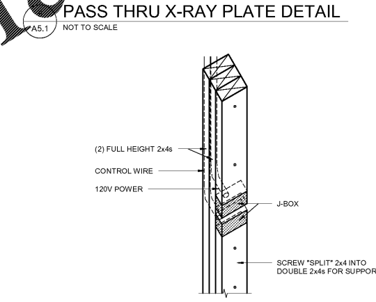
6 PASS THRU X-RAY PLATE DETAIL A5.1 NOT TO SCALE
