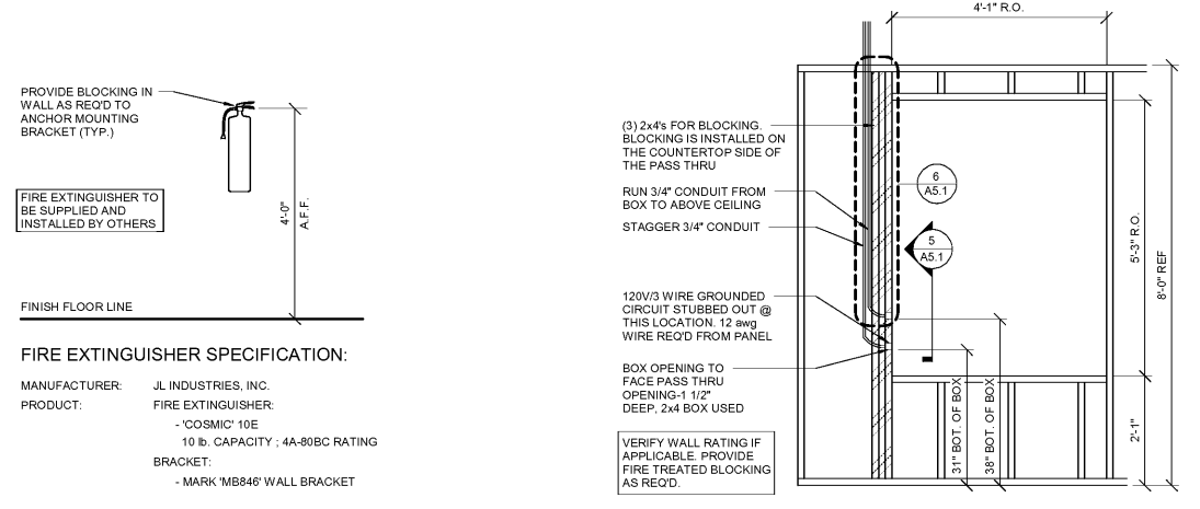
7 FIRE EXTINGUISHER DETAIL A5.1 SCALE: 1/2" = 1'-0"
