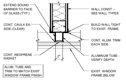
8 WALL CLOSURE DETAIL A5.1 NOT TO SCALE
