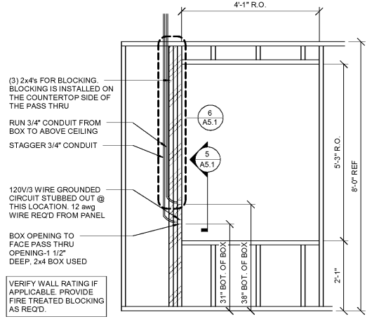
4 PASS THRU X-RAY A5.1 NOT TO SCALE
